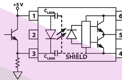
Figure 25 Recommended LED Drive Circuit for Ultra-High CMR Dead Time and Propagation Delay Specifications
